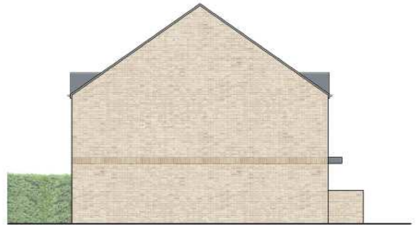
SOUTH ELEVATION
